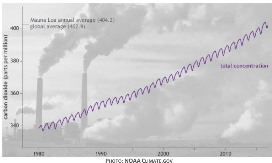
Monthly global carbon dioxide in parts per million from 1980-2016. xxxv
